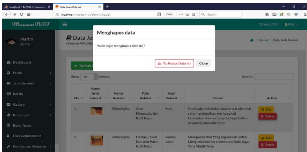
Gambar 4.18 Halaman Delete Data
