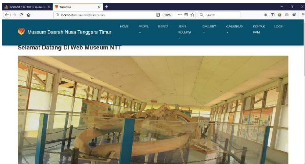
Gambar 4.2 Tampilan Welcome
